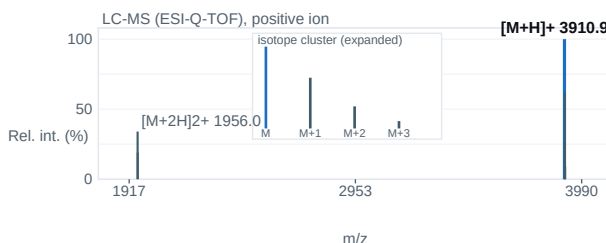
Fig. 2 — ESI-Q-TOF mass spectrum; base peak [M+H] + 3910.9 m/z.
