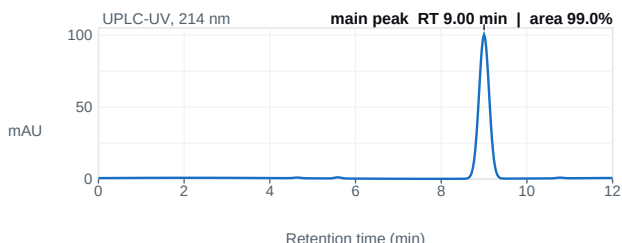
Fig. 1 — UPLC chromatogram; main peak 9.00 min, 99.0% area.
