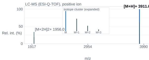
Fig. 2 — ESI-Q-TOF mass spectrum; base peak [M+H] + 3911.0 m/z.
