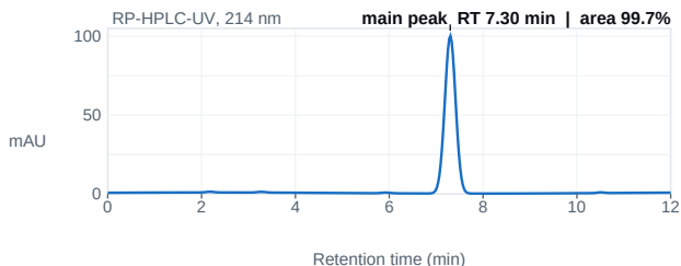
Fig. 1 — HPLC chromatogram; main peak 7.30 min, 99.7% area.
