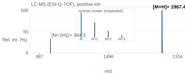
Fig. 2 — ESI-Q-TOF mass spectrum; base peak [M+H] + 1967.4 m/z.
