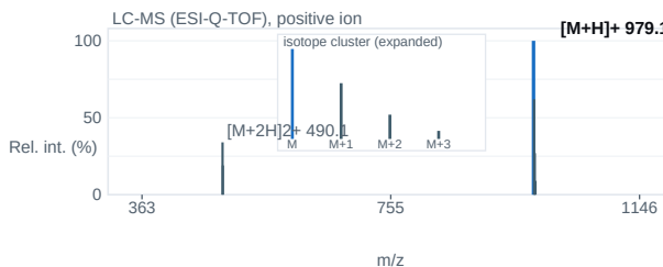
Fig. 2 — ESI-Q-TOF mass spectrum; base peak [M+H] + 979.1 m/z.
