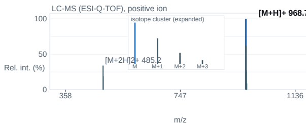
Fig. 2 — ESI-Q-TOF mass spectrum; base peak [M+H] + 968.7 m/z.
