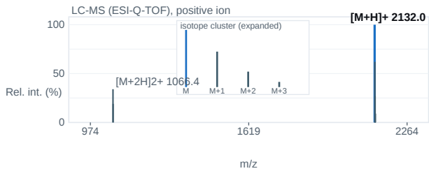
Fig. 2 — ESI-Q-TOF mass spectrum; base peak [M+H] + 2132.0 m/z.
