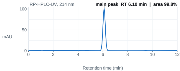
Fig. 1 — HPLC chromatogram; main peak 6.10 min, 99.8% area.
