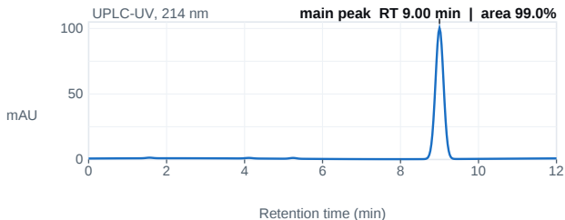
Fig. 1 — UPLC chromatogram; main peak 9.00 min, 99.0% area.
