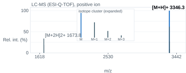
Fig. 2 — ESI-Q-TOF mass spectrum; base peak [M+H] + 3346.3 m/z.
