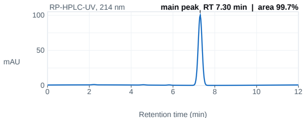
Fig. 1 — HPLC chromatogram; main peak 7.30 min, 99.7% area.
