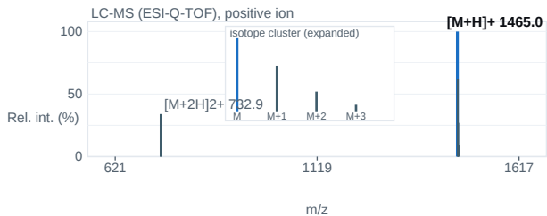
Fig. 2 — ESI-Q-TOF mass spectrum; base peak [M+H] + 1465.0 m/z.
