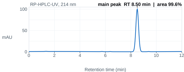
Fig. 1 — HPLC chromatogram; main peak 8.50 min, 99.6% area.
