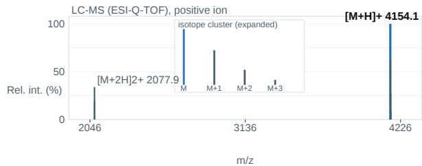
Fig. 2 — ESI-Q-TOF mass spectrum; base peak [M+H] + 4154.1 m/z.
