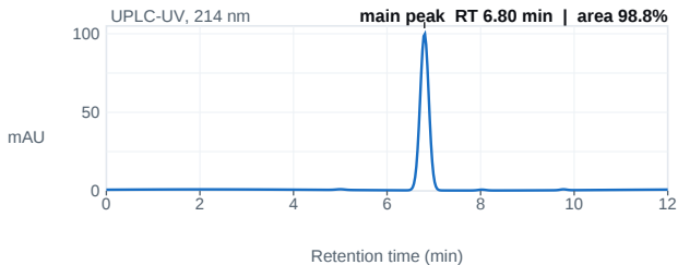
Fig. 1 — UPLC chromatogram; main peak 6.80 min, 98.8% area.
