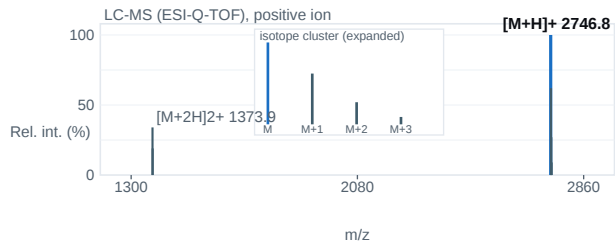
Fig. 2 — ESI-Q-TOF mass spectrum; base peak [M+H] + 2746.8 m/z.
