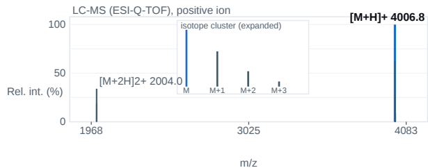
Fig. 2 — ESI-Q-TOF mass spectrum; base peak [M+H] + 4006.8 m/z.
