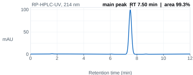
Fig. 1 — HPLC chromatogram; main peak 7.50 min, 99.3% area.
