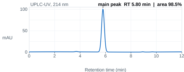
Fig. 1 — UPLC chromatogram; main peak 5.80 min, 98.5% area.
