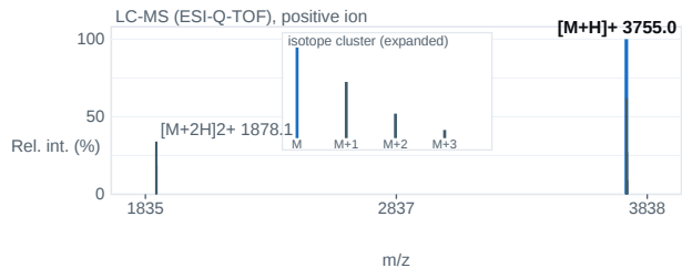
Fig. 2 — ESI-Q-TOF mass spectrum; base peak [M+H] + 3755.0 m/z.
