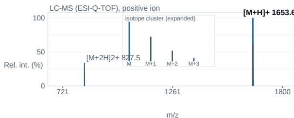
Fig. 2 — ESI-Q-TOF mass spectrum; base peak [M+H] + 1653.6 m/z.
