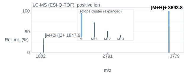
Fig. 2 — ESI-Q-TOF mass spectrum; base peak [M+H] + 3693.8 m/z.
