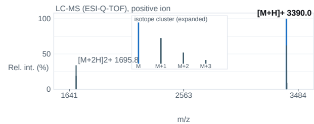
Fig. 2 — ESI-Q-TOF mass spectrum; base peak [M+H] + 3390.0 m/z.
