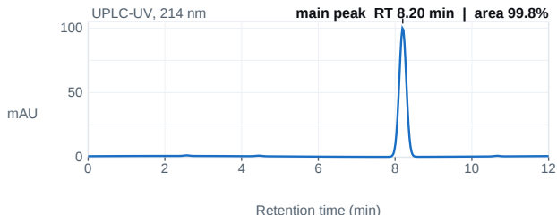
Fig. 1 — UPLC chromatogram; main peak 8.20 min, 99.8% area.
