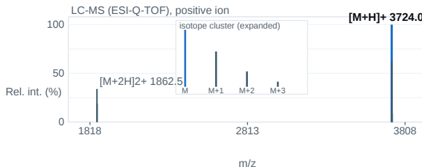
Fig. 2 — ESI-Q-TOF mass spectrum; base peak [M+H] + 3724.0 m/z.
