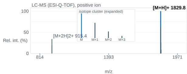
Fig. 2 — ESI-Q-TOF mass spectrum; base peak [M+H] + 1829.8 m/z.
