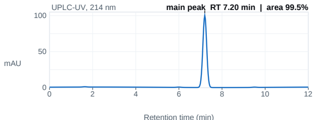
Fig. 1 — UPLC chromatogram; main peak 7.20 min, 99.5% area.
