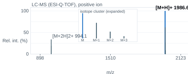
Fig. 2 — ESI-Q-TOF mass spectrum; base peak [M+H] + 1986.6 m/z.
