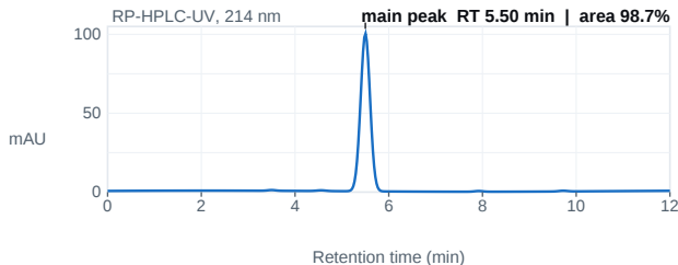
Fig. 1 — HPLC chromatogram; main peak 5.50 min, 98.7% area.
