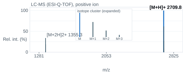
Fig. 2 — ESI-Q-TOF mass spectrum; base peak [M+H] + 2709.8 m/z.
