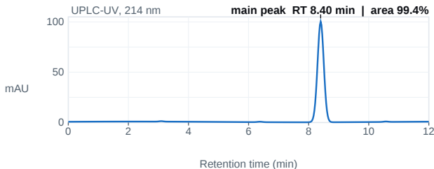
Fig. 1 — UPLC chromatogram; main peak 8.40 min, 99.4% area.
