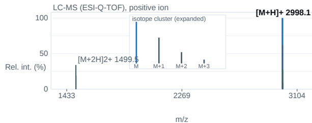
Fig. 2 — ESI-Q-TOF mass spectrum; base peak [M+H] + 2998.1 m/z.
