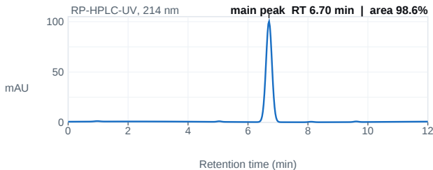
Fig. 1 — HPLC chromatogram; main peak 6.70 min, 98.6% area.
