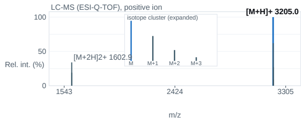
Fig. 2 — ESI-Q-TOF mass spectrum; base peak [M+H] + 3205.0 m/z.
