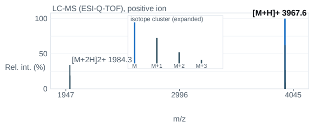
Fig. 2 — ESI-Q-TOF mass spectrum; base peak [M+H] + 3967.6 m/z.
