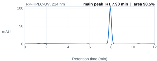
Fig. 1 — HPLC chromatogram; main peak 7.90 min, 98.5% area.
