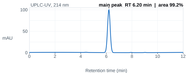
Fig. 1 — UPLC chromatogram; main peak 6.20 min, 99.2% area.
