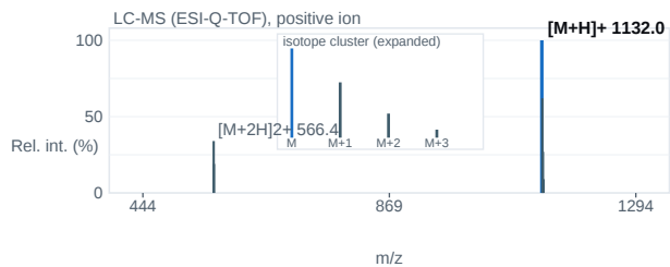
Fig. 2 — ESI-Q-TOF mass spectrum; base peak [M+H] + 1132.0 m/z.
