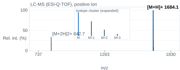
Fig. 2 — ESI-Q-TOF mass spectrum; base peak [M+H] + 1684.1 m/z.
