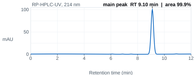
Fig. 1 — HPLC chromatogram; main peak 9.10 min, 99.9% area.
