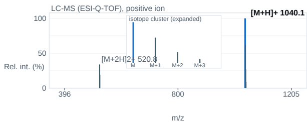
Fig. 2 — ESI-Q-TOF mass spectrum; base peak [M+H] + 1040.1 m/z.
