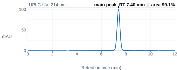
Fig. 1 — UPLC chromatogram; main peak 7.40 min, 99.1% area.
