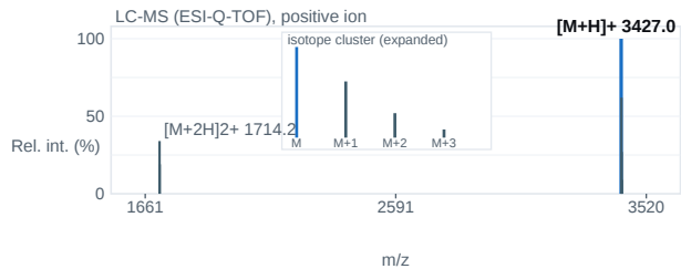
Fig. 2 — ESI-Q-TOF mass spectrum; base peak [M+H] + 3427.0 m/z.
