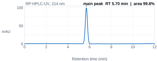
Fig. 1 — HPLC chromatogram; main peak 5.70 min, 99.8% area.
