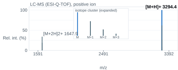
Fig. 2 — ESI-Q-TOF mass spectrum; base peak [M+H] + 3294.4 m/z.
