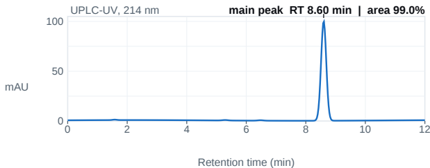
Fig. 1 — UPLC chromatogram; main peak 8.60 min, 99.0% area.
