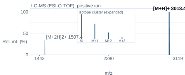
Fig. 2 — ESI-Q-TOF mass spectrum; base peak [M+H] + 3013.4 m/z.
