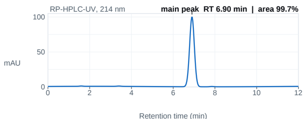
Fig. 1 — HPLC chromatogram; main peak 6.90 min, 99.7% area.
