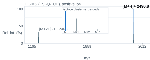
Fig. 2 — ESI-Q-TOF mass spectrum; base peak [M+H] + 2490.8 m/z.
