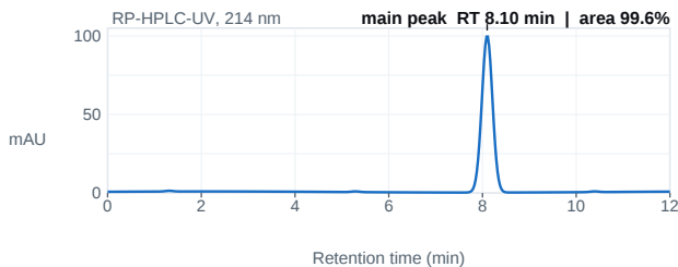
Fig. 1 — HPLC chromatogram; main peak 8.10 min, 99.6% area.
