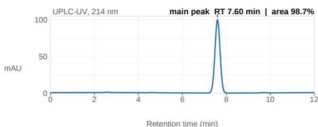
Fig. 1 — UPLC chromatogram; main peak 7.60 min, 98.7% area.
