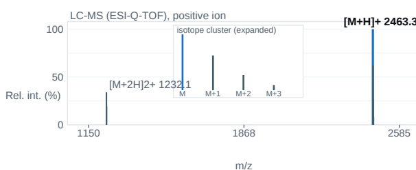
Fig. 2 — ESI-Q-TOF mass spectrum; base peak [M+H] + 2463.3 m/z.
