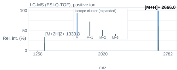
Fig. 2 — ESI-Q-TOF mass spectrum; base peak [M+H] + 2666.0 m/z.
