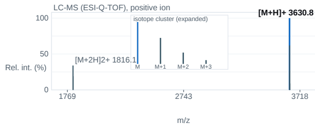
Fig. 2 — ESI-Q-TOF mass spectrum; base peak [M+H] + 3630.8 m/z.
