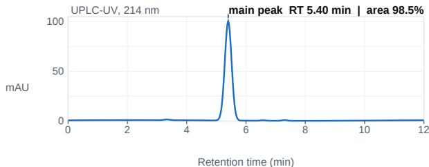
Fig. 1 — UPLC chromatogram; main peak 5.40 min, 98.5% area.
