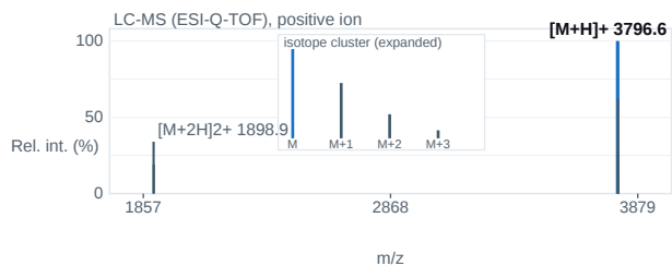
Fig. 2 — ESI-Q-TOF mass spectrum; base peak [M+H] + 3796.6 m/z.
