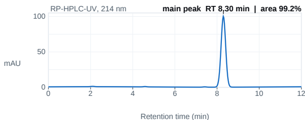
Fig. 1 — HPLC chromatogram; main peak 8.30 min, 99.2% area.
