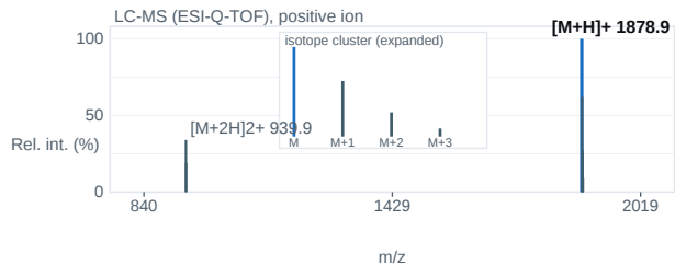
Fig. 2 — ESI-Q-TOF mass spectrum; base peak [M+H] + 1878.9 m/z.
