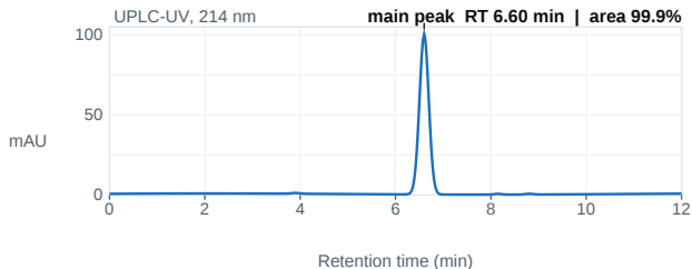
Fig. 1 — UPLC chromatogram; main peak 6.60 min, 99.9% area.
