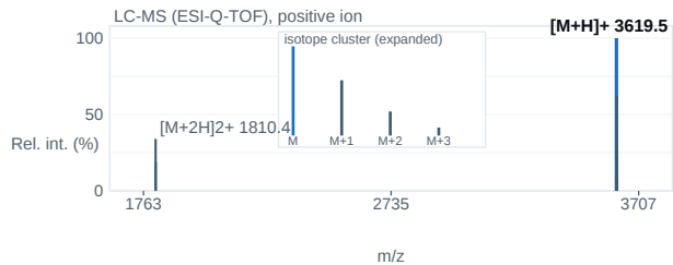
Fig. 2 — ESI-Q-TOF mass spectrum; base peak [M+H] + 3619.5 m/z.
