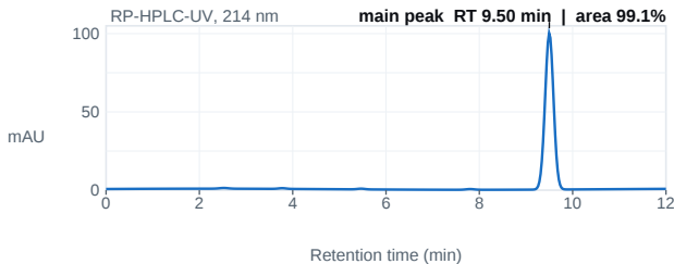
Fig. 1 — HPLC chromatogram; main peak 9.50 min, 99.1% area.
