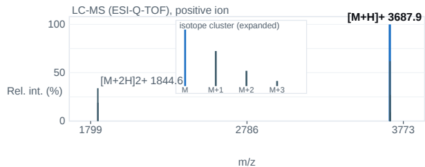
Fig. 2 — ESI-Q-TOF mass spectrum; base peak [M+H] + 3687.9 m/z.
