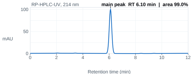
Fig. 1 — HPLC chromatogram; main peak 6.10 min, 99.0% area.
