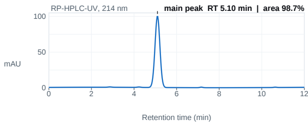
Fig. 1 — HPLC chromatogram; main peak 5.10 min, 98.7% area.
