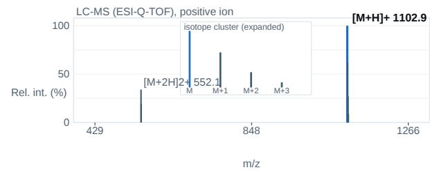
Fig. 2 — ESI-Q-TOF mass spectrum; base peak [M+H] + 1102.9 m/z.
