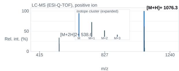
Fig. 2 — ESI-Q-TOF mass spectrum; base peak [M+H] + 1076.3 m/z.
