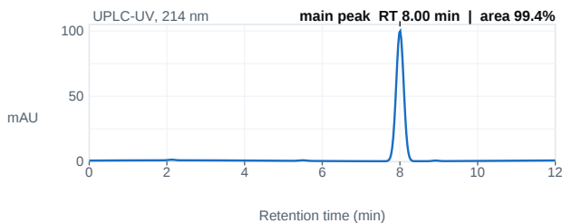
Fig. 1 — UPLC chromatogram; main peak 8.00 min, 99.4% area.
