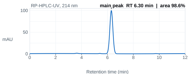
Fig. 1 — HPLC chromatogram; main peak 6.30 min, 98.6% area.
