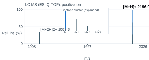
Fig. 2 — ESI-Q-TOF mass spectrum; base peak [M+H] + 2196.0 m/z.
