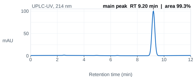
Fig. 1 — UPLC chromatogram; main peak 9.20 min, 99.3% area.
