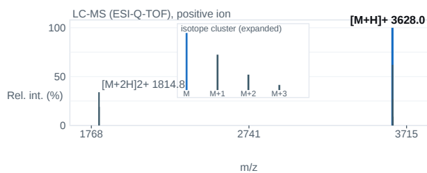
Fig. 2 — ESI-Q-TOF mass spectrum; base peak [M+H] + 3628.0 m/z.
