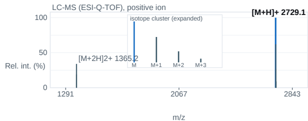
Fig. 2 — ESI-Q-TOF mass spectrum; base peak [M+H] + 2729.1 m/z.
