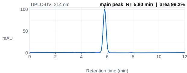
Fig. 1 — UPLC chromatogram; main peak 5.80 min, 99.2% area.
