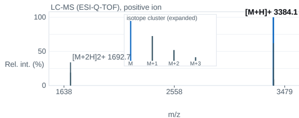
Fig. 2 — ESI-Q-TOF mass spectrum; base peak [M+H] + 3384.1 m/z.
