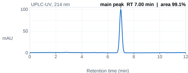
Fig. 1 — UPLC chromatogram; main peak 7.00 min, 99.1% area.
