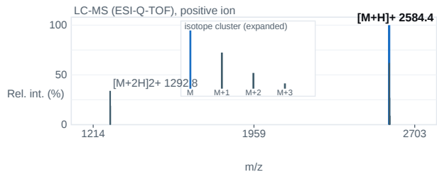
Fig. 2 — ESI-Q-TOF mass spectrum; base peak [M+H] + 2584.4 m/z.
