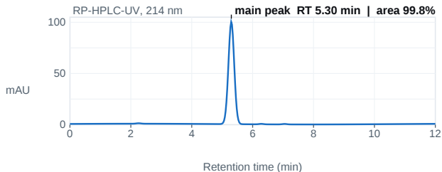
Fig. 1 — HPLC chromatogram; main peak 5.30 min, 99.8% area.
