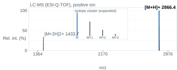
Fig. 2 — ESI-Q-TOF mass spectrum; base peak [M+H] + 2866.4 m/z.
