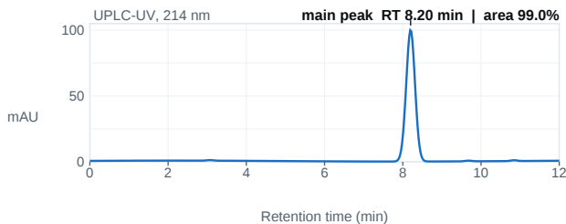
Fig. 1 — UPLC chromatogram; main peak 8.20 min, 99.0% area.
