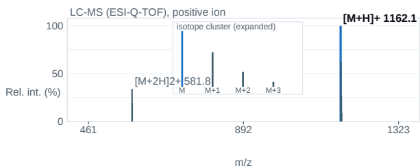
Fig. 2 — ESI-Q-TOF mass spectrum; base peak [M+H] + 1162.1 m/z.
