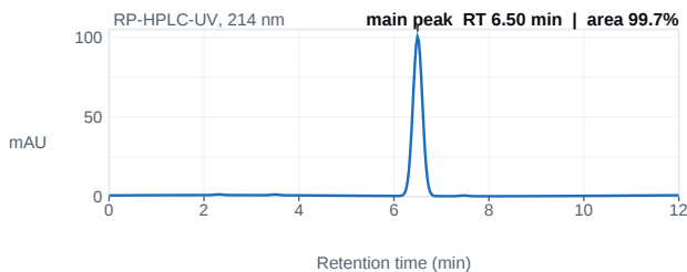
Fig. 1 — HPLC chromatogram; main peak 6.50 min, 99.7% area.
