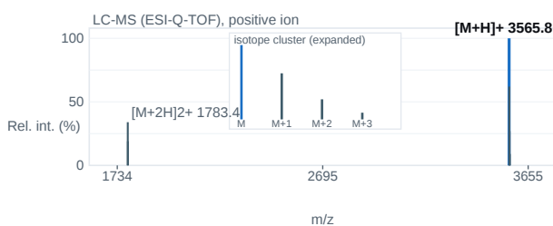
Fig. 2 — ESI-Q-TOF mass spectrum; base peak [M+H] + 3565.8 m/z.
