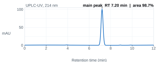
Fig. 1 — UPLC chromatogram; main peak 7.20 min, 98.7% area.
