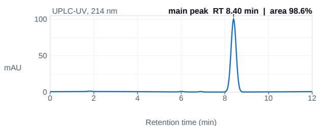
Fig. 1 — UPLC chromatogram; main peak 8.40 min, 98.6% area.
