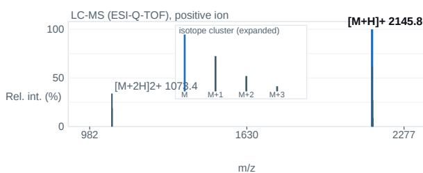
Fig. 2 — ESI-Q-TOF mass spectrum; base peak [M+H] + 2145.8 m/z.
