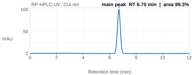
Fig. 1 — HPLC chromatogram; main peak 6.70 min, 99.3% area.
