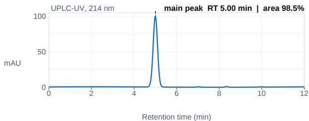
Fig. 1 — UPLC chromatogram; main peak 5.00 min, 98.5% area.
