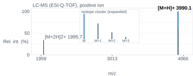
Fig. 2 — ESI-Q-TOF mass spectrum; base peak [M+H] + 3990.1 m/z.
