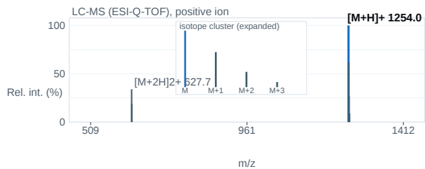
Fig. 2 — ESI-Q-TOF mass spectrum; base peak [M+H] + 1254.0 m/z.
