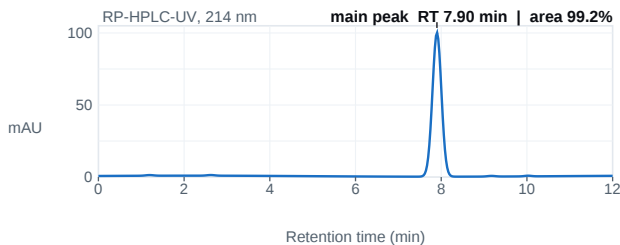
Fig. 1 — HPLC chromatogram; main peak 7.90 min, 99.2% area.
